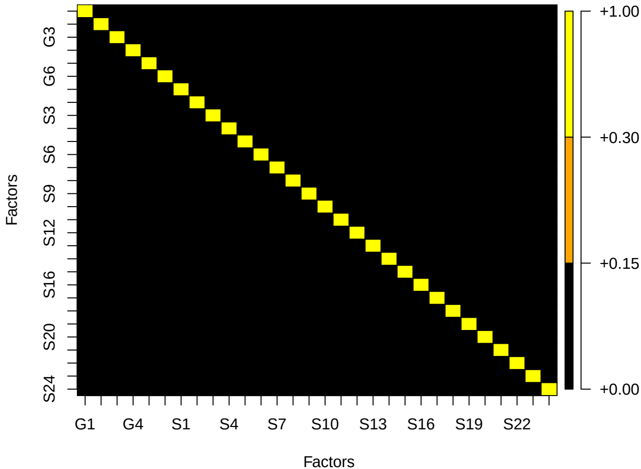
Absolute value of factor correlations (geomin + geomin)
